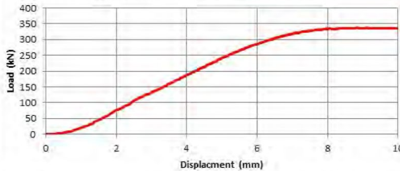
Load vs. Displacement Typical Test Curve D1515236
